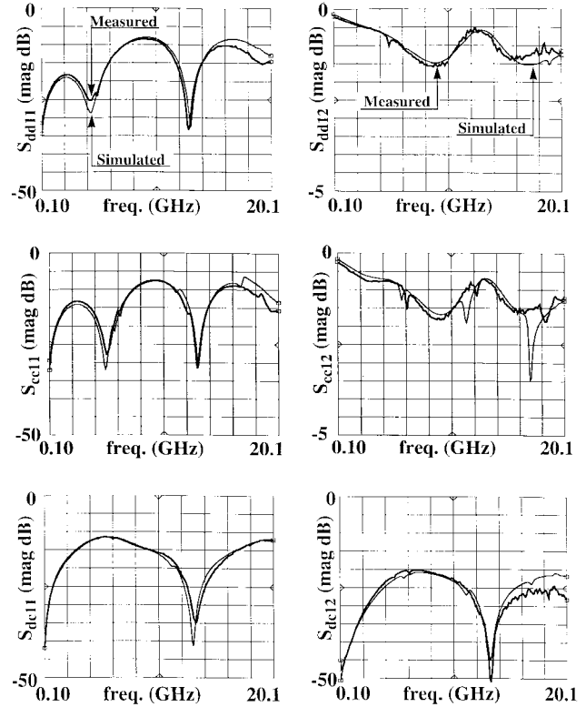
Fig. 6. Selected measured and simulated mixed-mode s -parameters of the asymmetric-stepped transmission-line pair. The heavy line indicates measured data, while the lighter line indicates simulated data.
