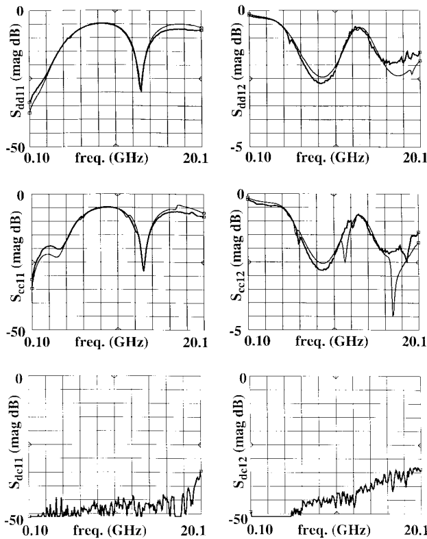
Fig. 7. Selected measured and simulated mixed-mode s -parameters of the symmetric-stepped transmission-line pair. The heavy line indicates measured data, while the lighter line indicates simulated data.
