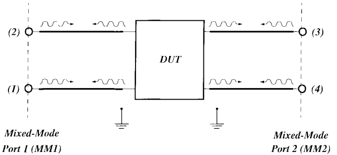
Fig. 1. Schematic of general two-port differential device.
