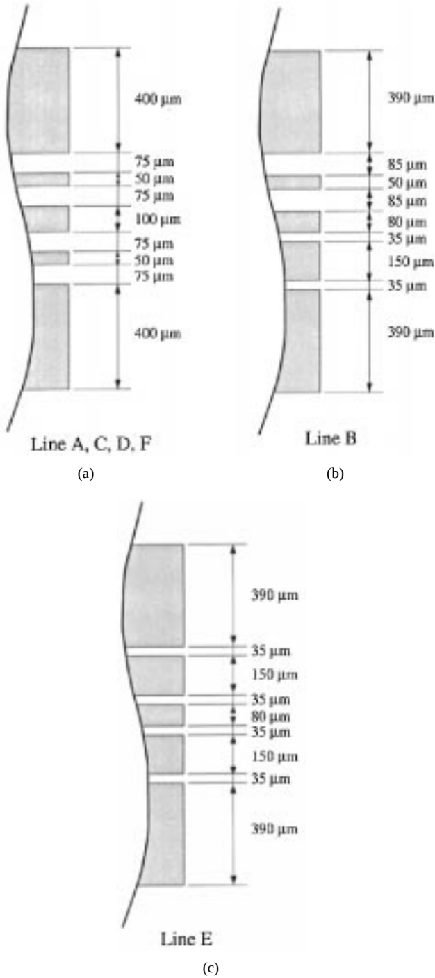
Fig. 5. Detail of layouts showing dimensions of (a) transmission-line pair A, C, D, F, (b) transmission-line pair B, and (c) transmission-line pair E.
