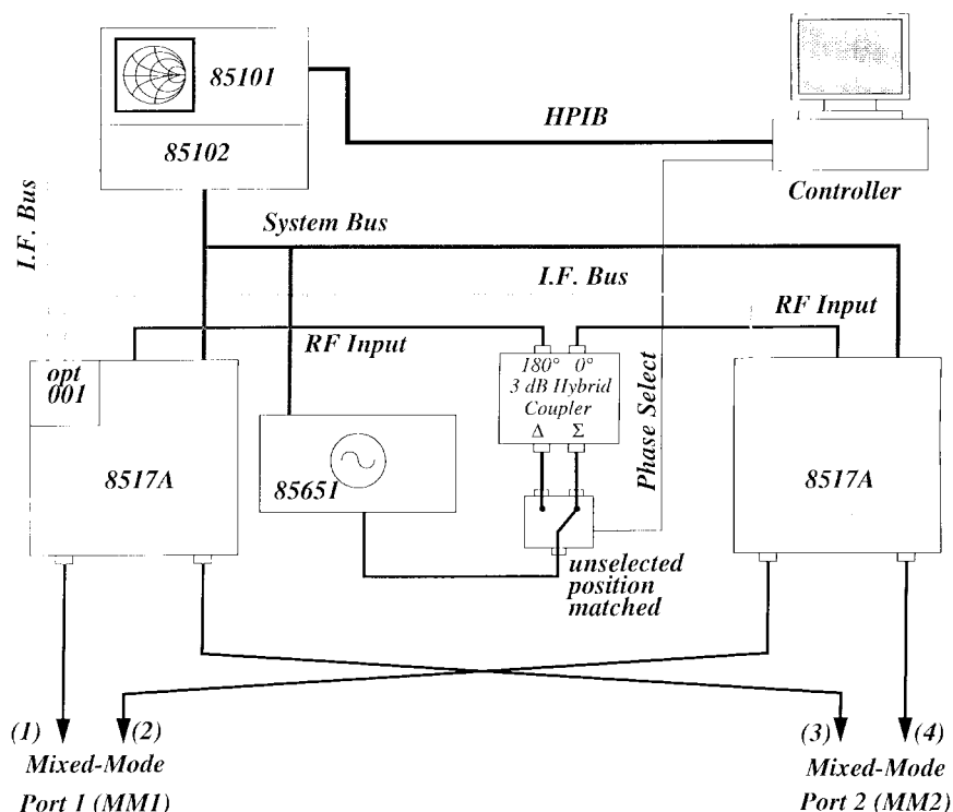
Fig. 2. Block diagram of PMVNA as implemented.
