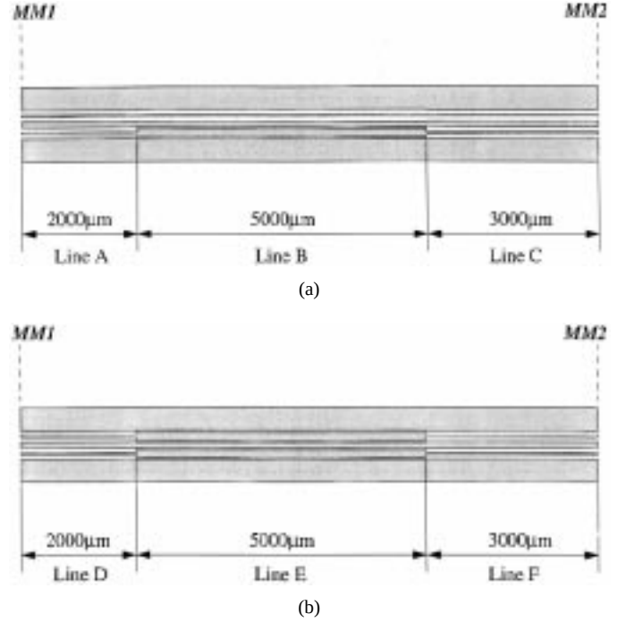
Fig. 4. Layout of the measured differential structures. (a) Transmission-line pair with an asymmetric step in characteristic impedance. (b) Transmission-line pair with a symmetric step in characteristic impedance.
