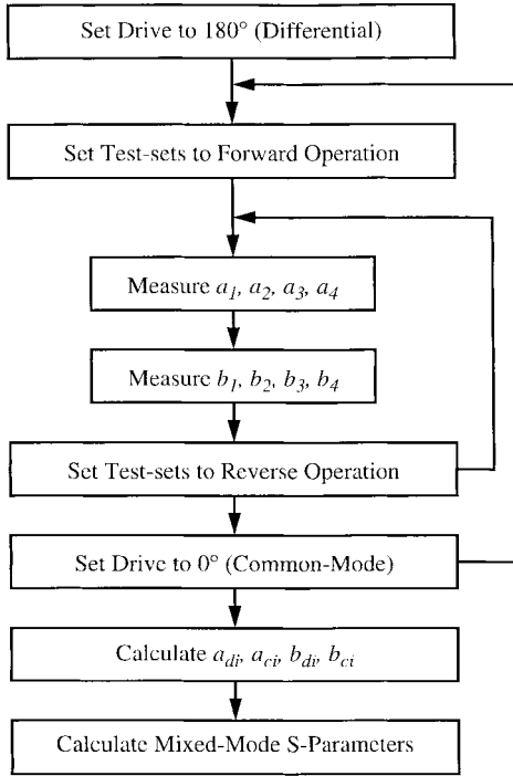
Fig. 3. Flow chart of the operation of the PMVNA.
